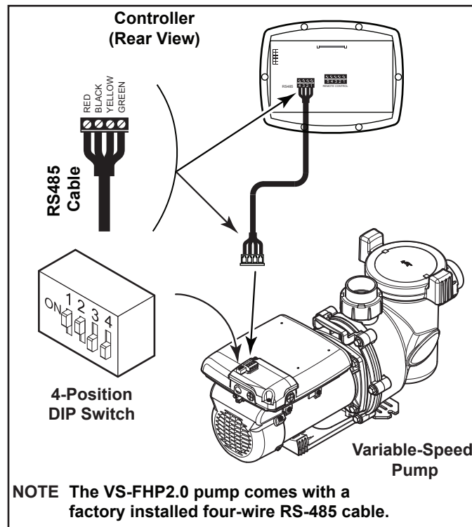
Figure 9. Wiring Variable-Speed Controller (JEP-R) to VS-FHP2.0 Pump
