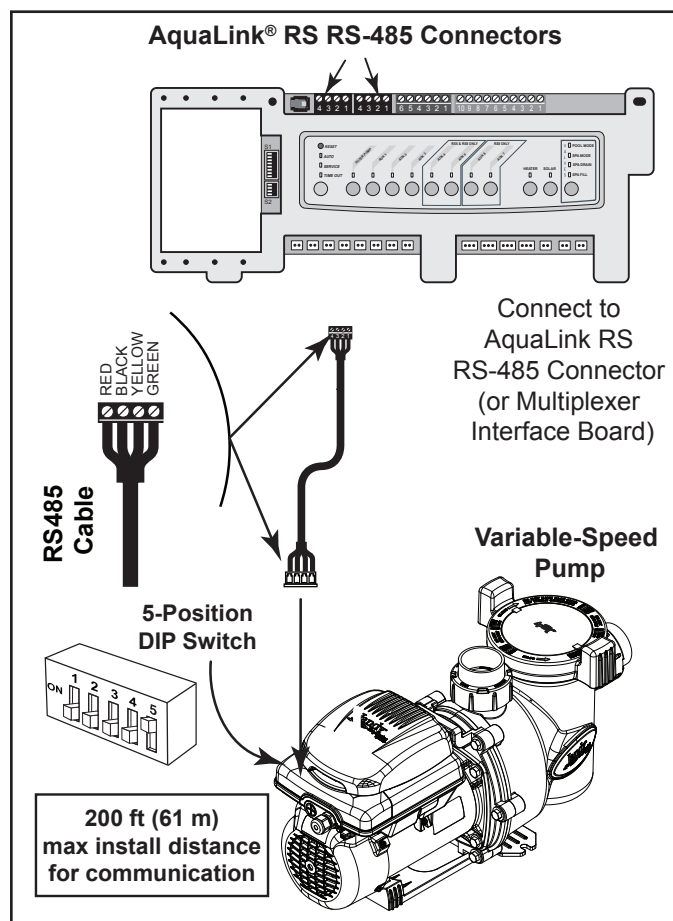
Figure 7. Wiring AquaLink RS Controller or AquaLink PDA to VS-FHP1.0 Pump
