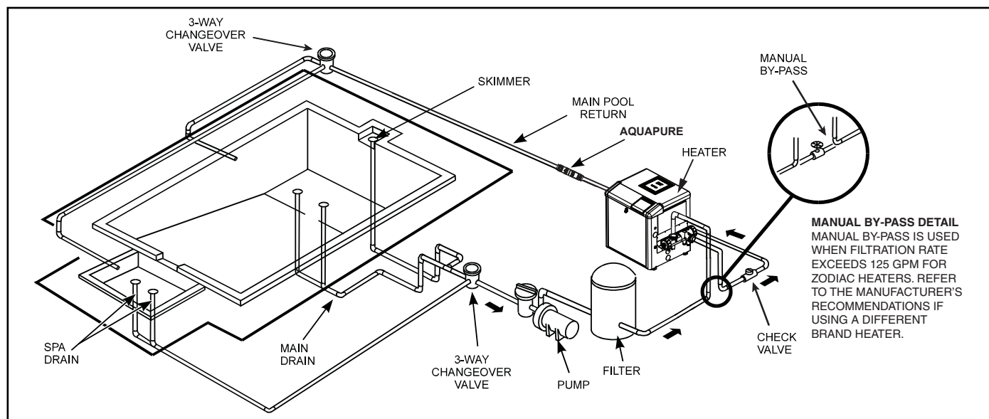
Figure 2. Typical Piping Installation
