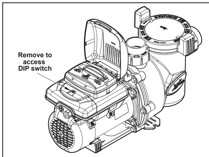
Figure 11. DIP Switch access cover on VS-FHP1.0 Motor
