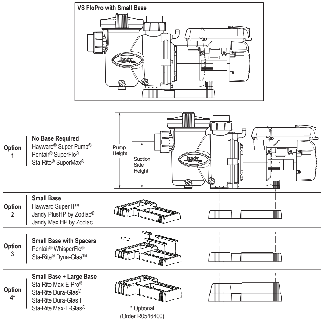
Figure 3. VS FloPro Pump and Base Options
