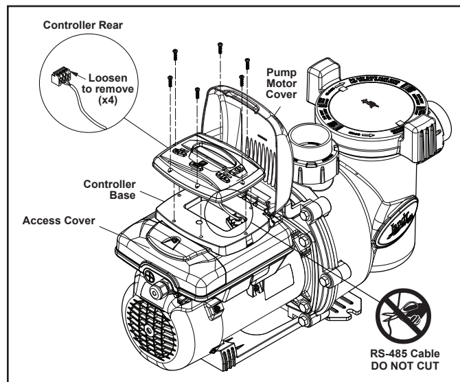
Figure 8. Disconnect Variable-Speed Controller from VS-FHP1.0 Pump
