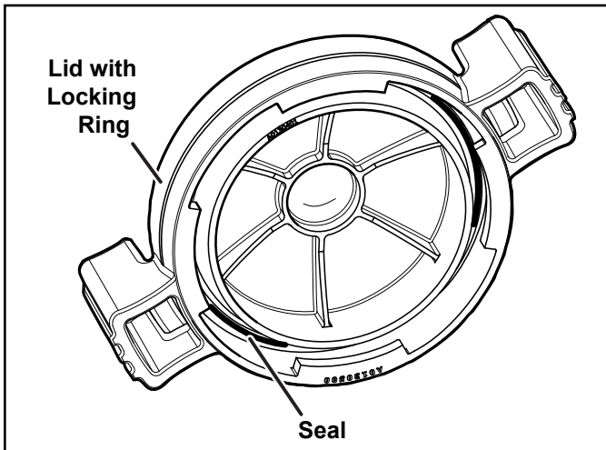
Figure 15. O-ring in Lid Assembly
