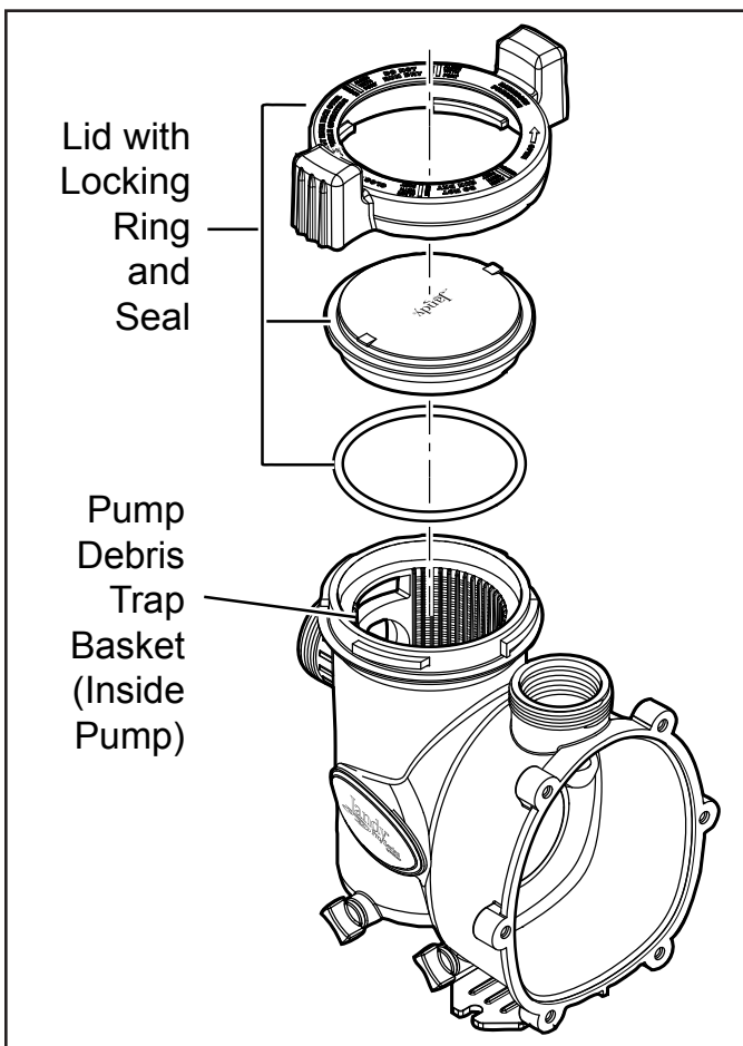
Figure 16. Exploded View of Pump
