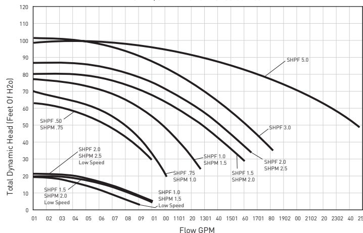
SHPF/SHPM Performance Curves
